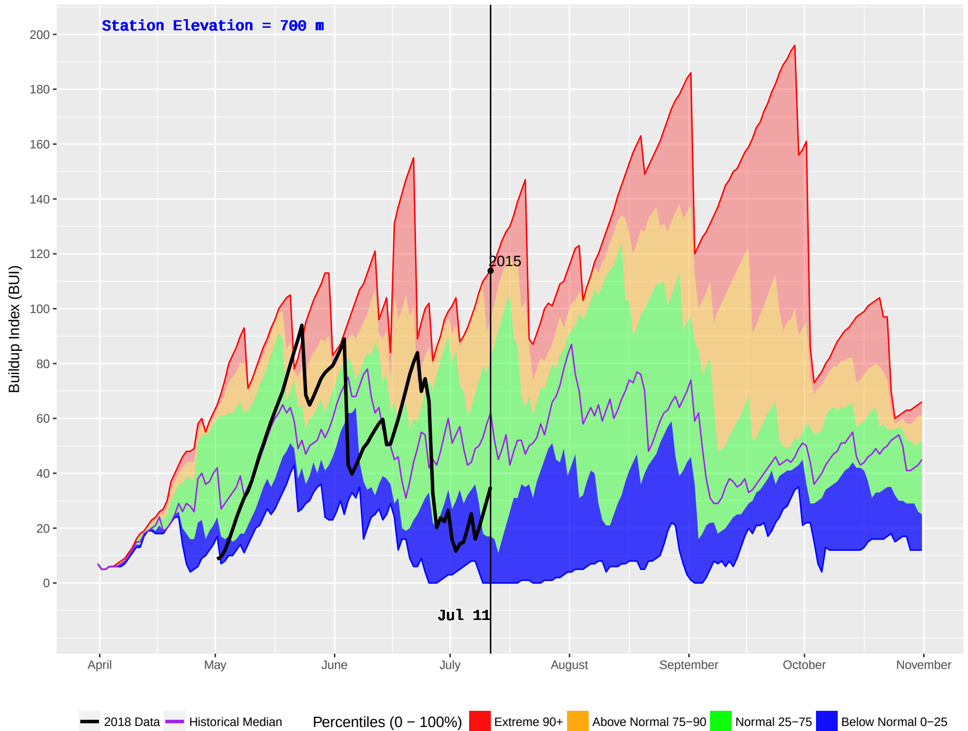
OSBORN (1045) : Historical (2009–2016) and Current (2018) Noon Buildup Index (BUI)
