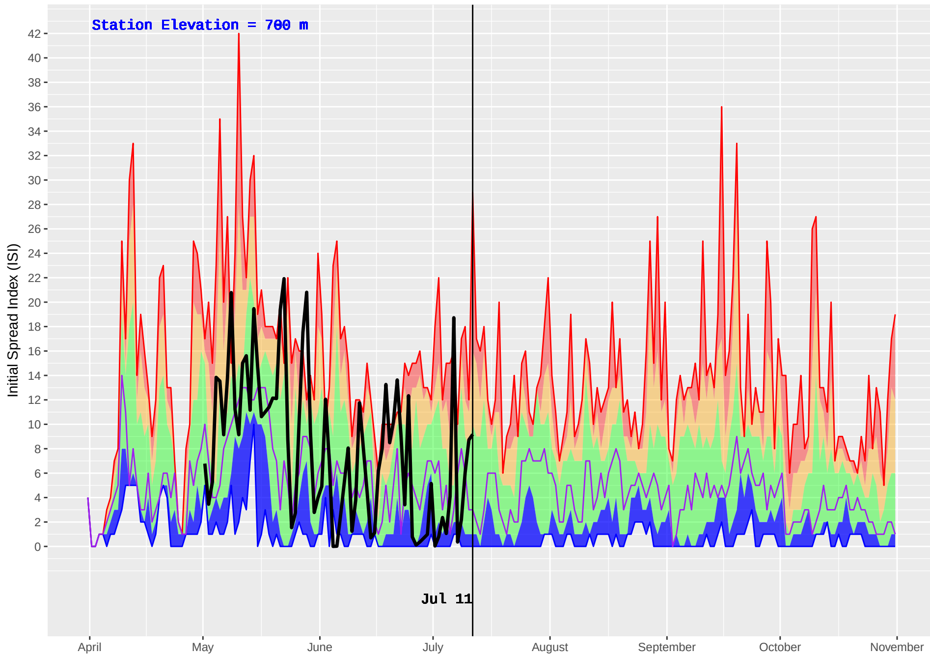
OSBORN (1045) : Historical (2009–2016) and Current (2018) Noon Initial Spread Index (ISI)
