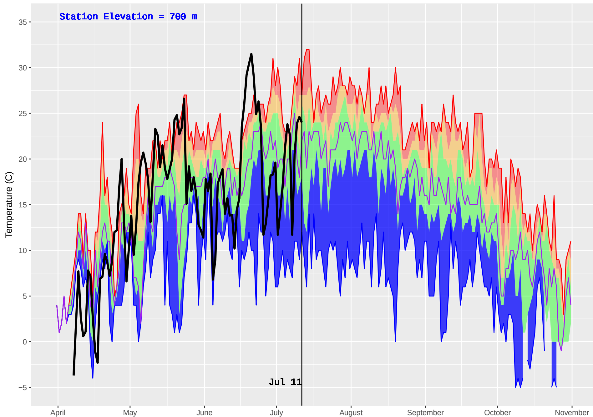
OSBORN (1045) : Historical (2009–2016) and Current (2018) Noon Temperature
